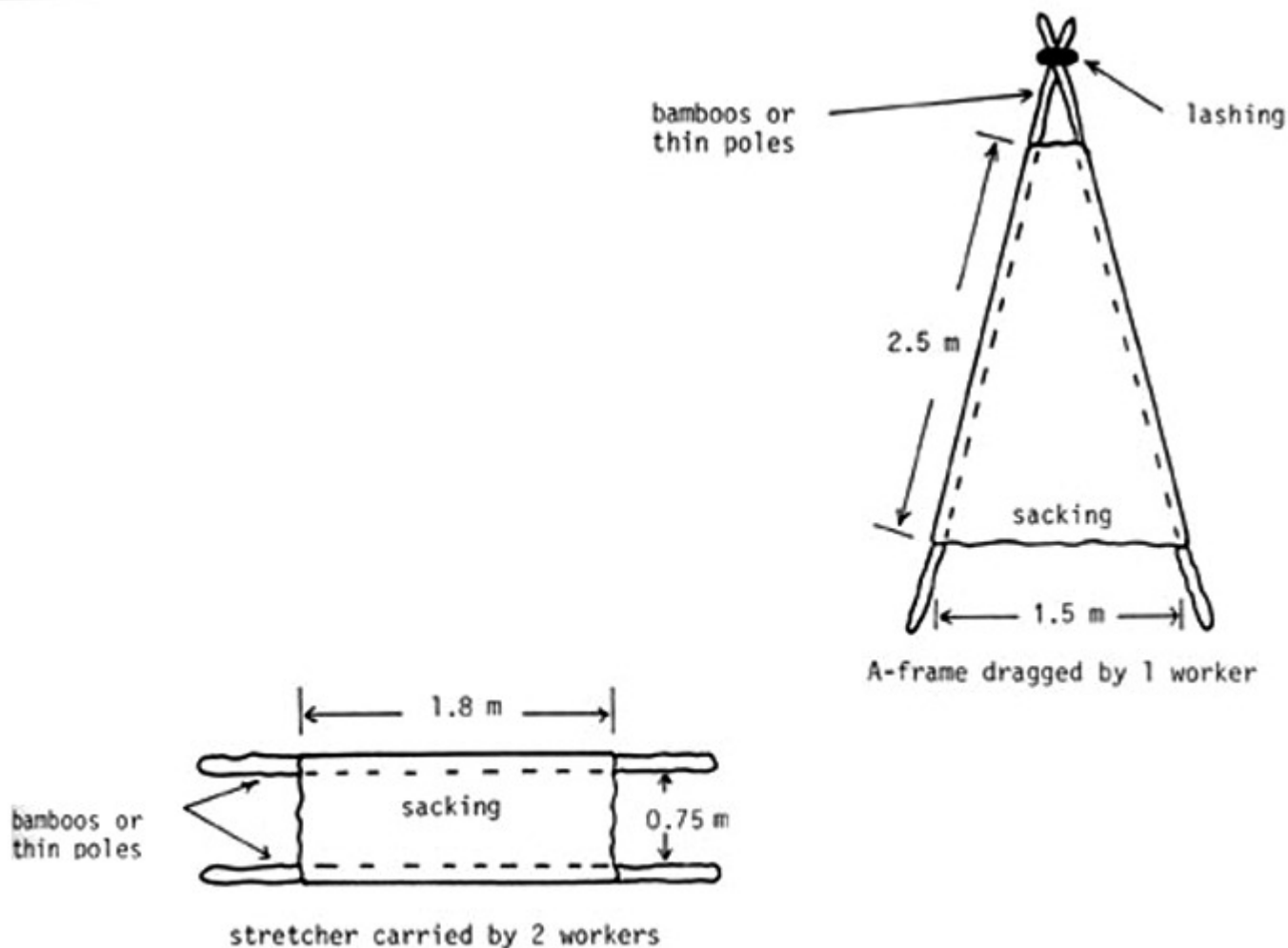
Figure 27 Stretchers for carrying wastes
