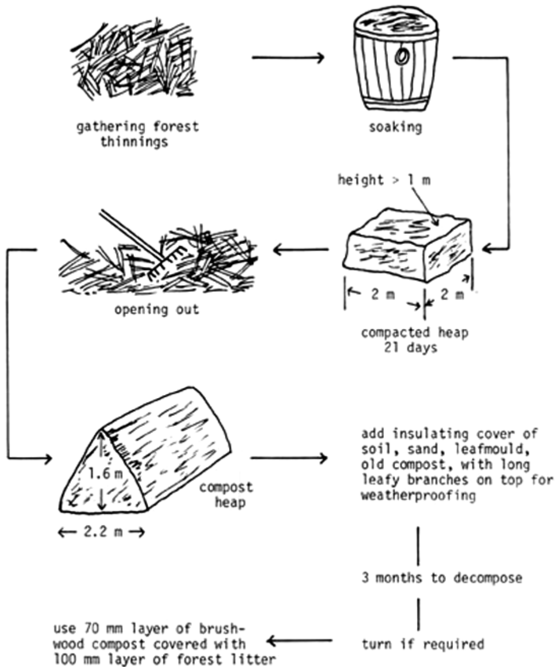
Figure 26 Brushwood composting system
