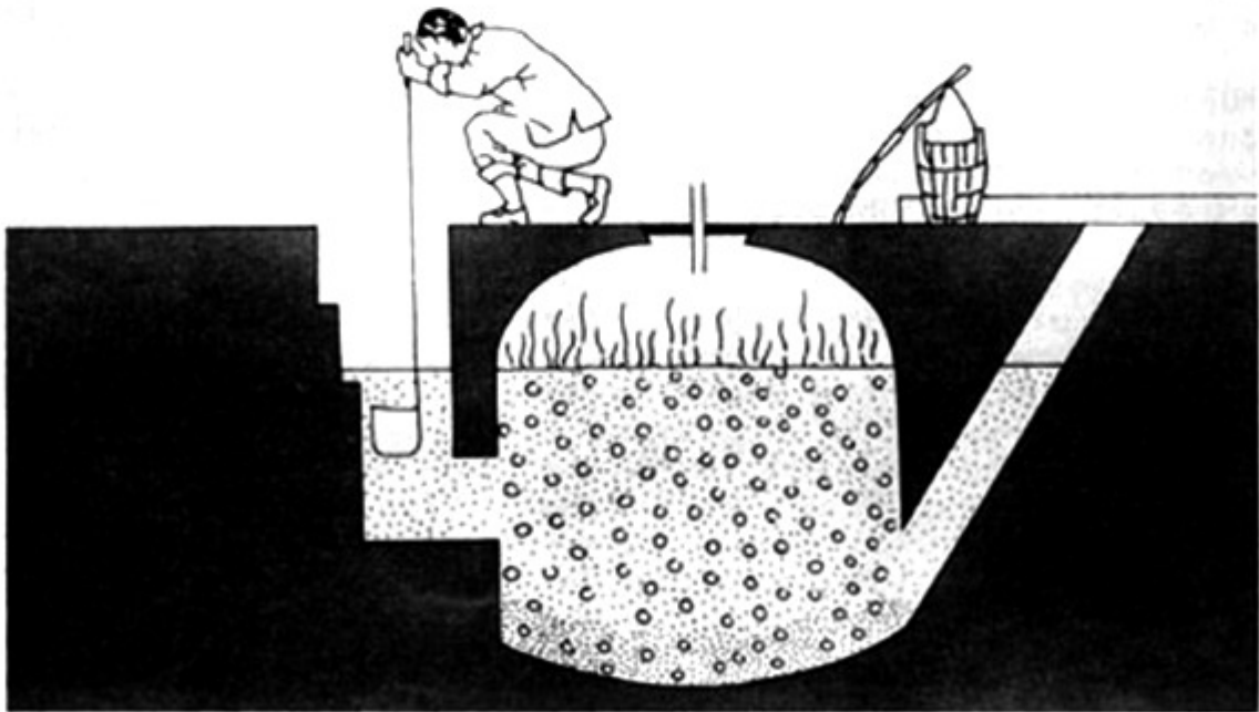
Plate 31 Removal of biogas sludge from the sludge outlet pipe Source: FAO filmstrip Biogas in China
