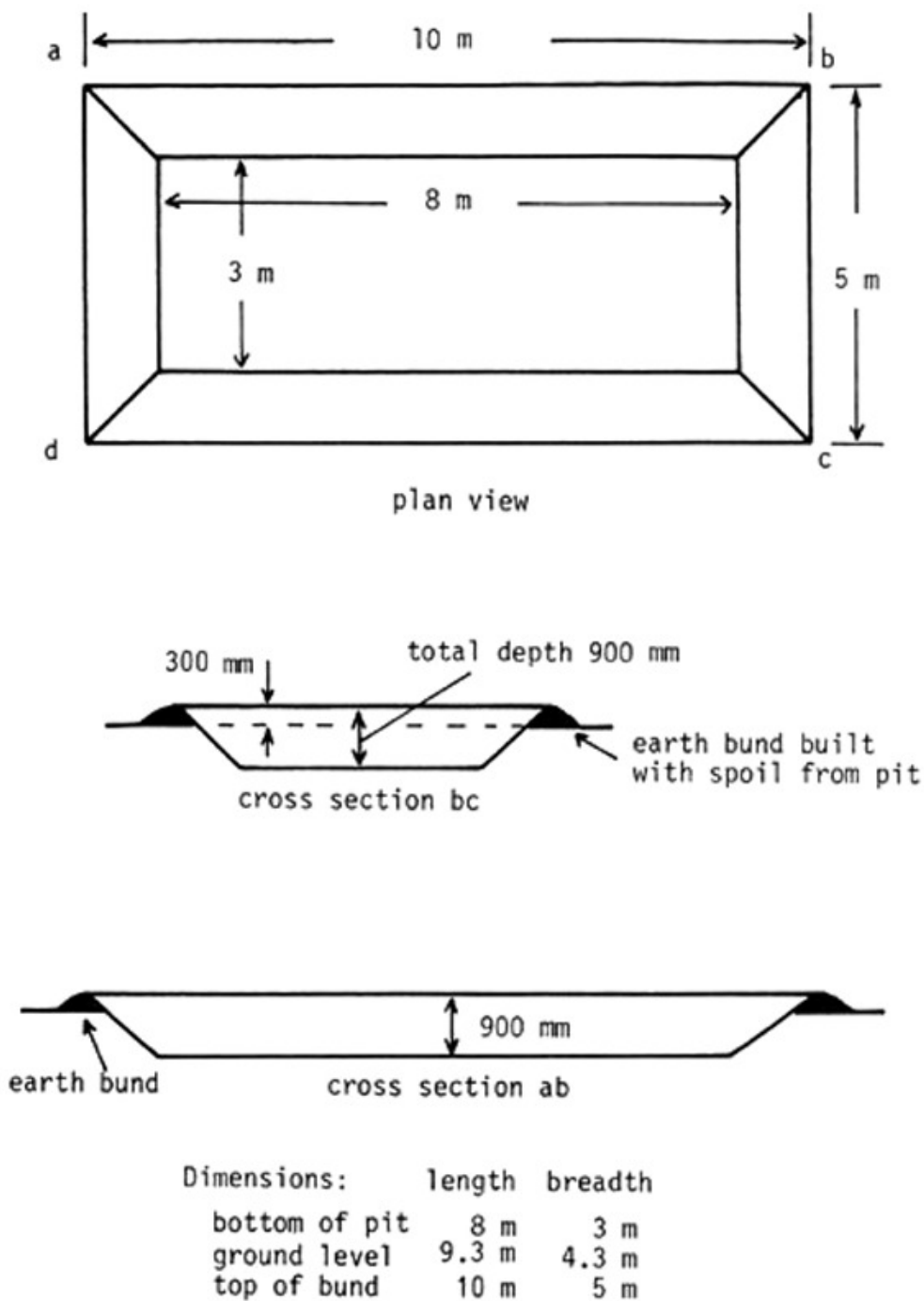
Figure 21 Details of a compost pit
